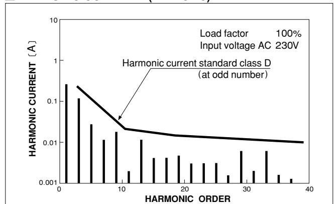
HARMONIC CURRENT (PAA75F-5)
