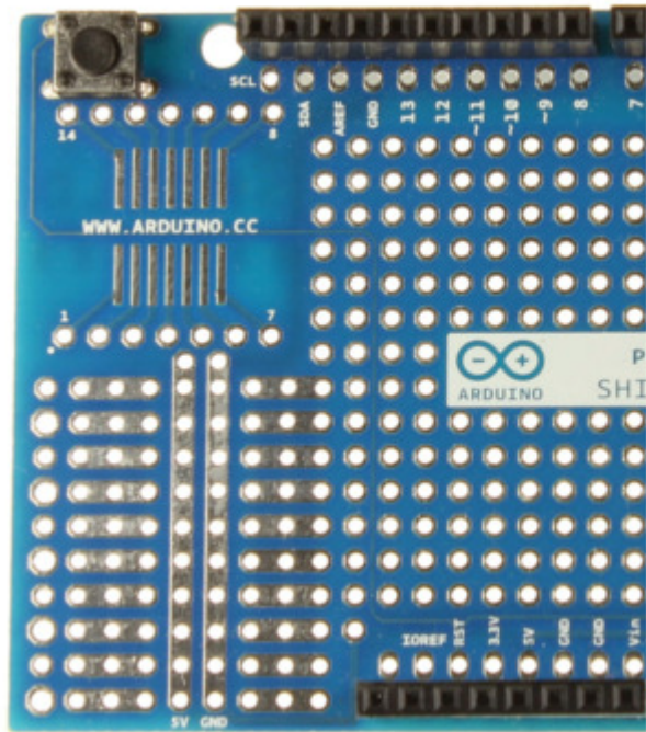
Proto Shield R3 mounted Front
