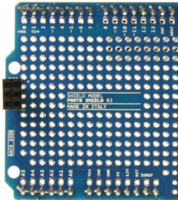
Proto Shield R3 mounted Back
