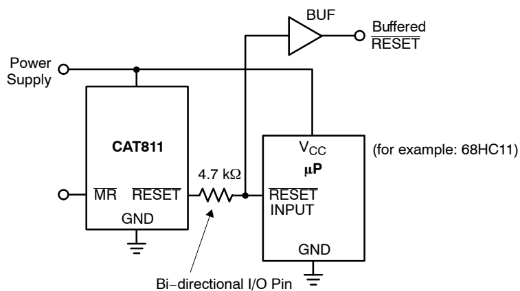
Figure 10. Bi-directional Reset Pin Interfacing
