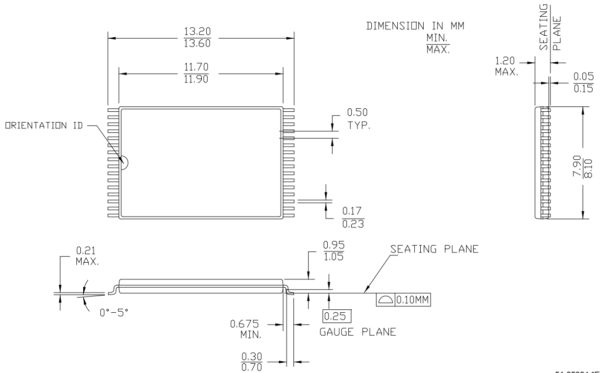
Figure 7. 32-pin Shrunk Thin Small Outline Package (8 x 13.4 mm) (51-85094)
