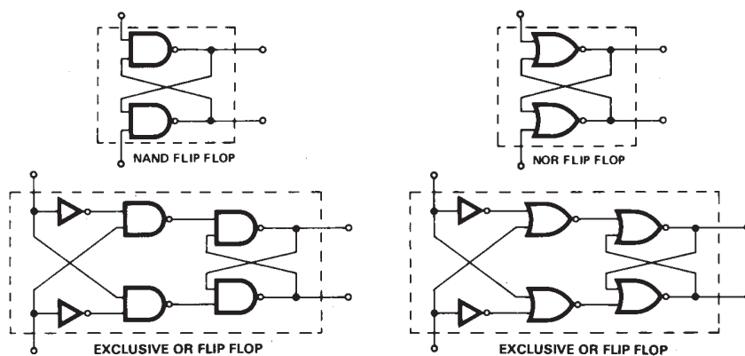
Figure d. Flip-Flop Configurations.
