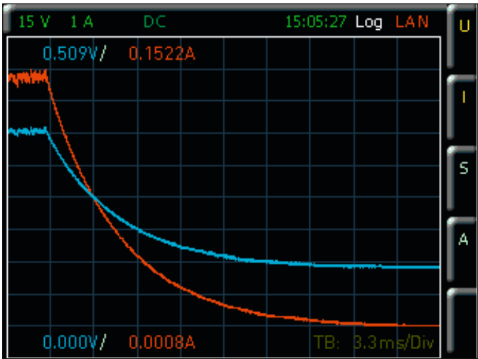
Inrush function.
