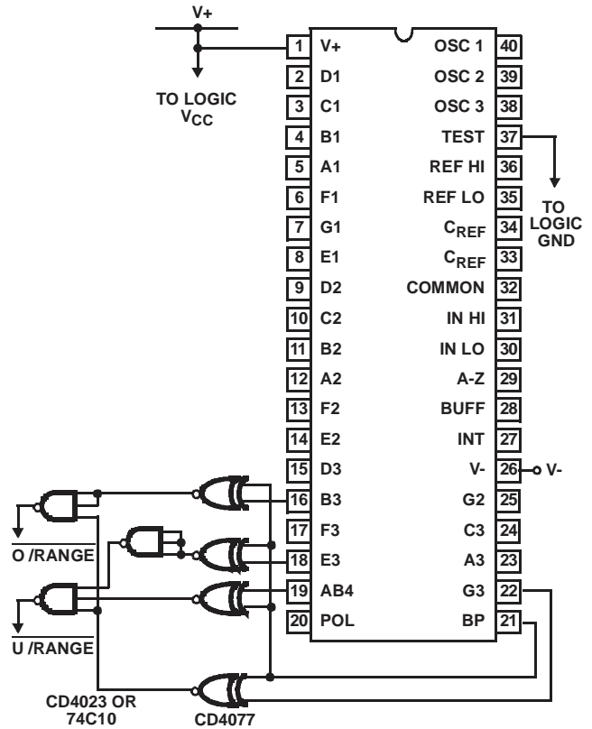
FIGURE 11. CIRCUIT FOR DEVELOPING UNDERANGE AND OVERANGE SIGNAL FROM ICL7136 OUTPUTS
