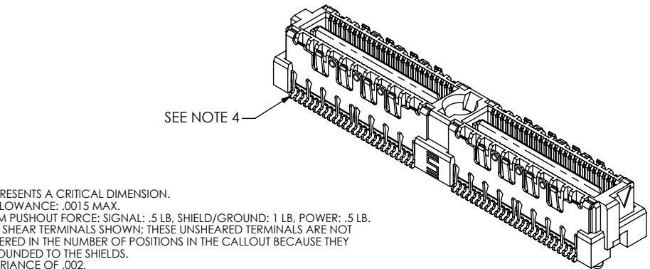
FIG 1 -06.75 LEAD STYLE (QMSS-032-06.75-X-D-DP-A SHOWN) (MATED HEIGHT WITH QFSS-04.25: .433 [11.00] REF)
