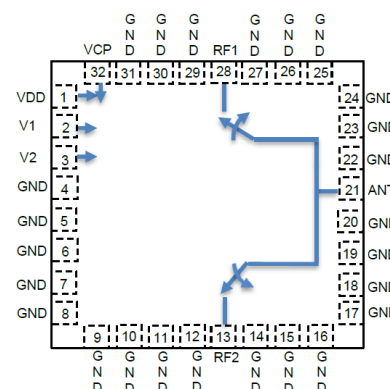
Figure 2 Function Block Diagram (Top View)
