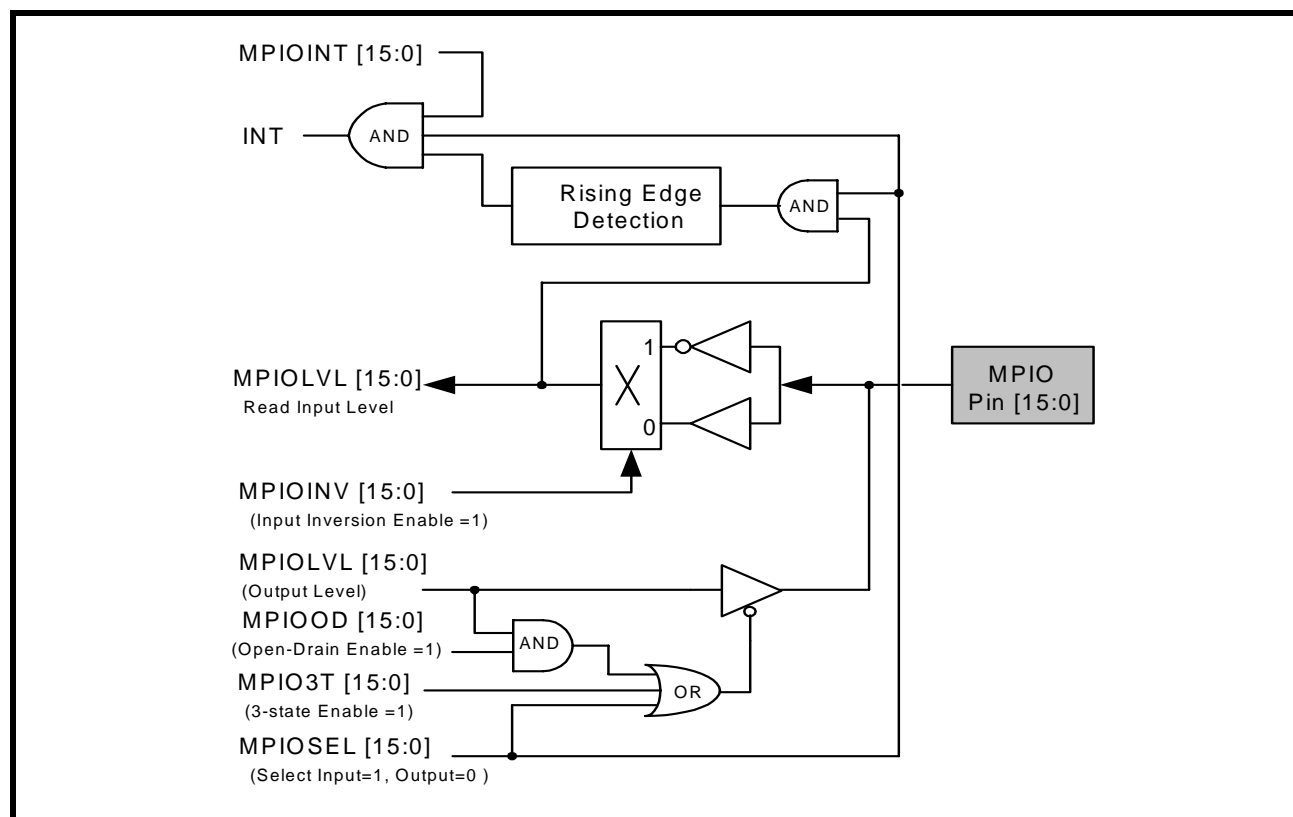
FIGURE 8. MULTIPURPOSE INPUT/OUTPUT INTERNAL CIRCUIT
